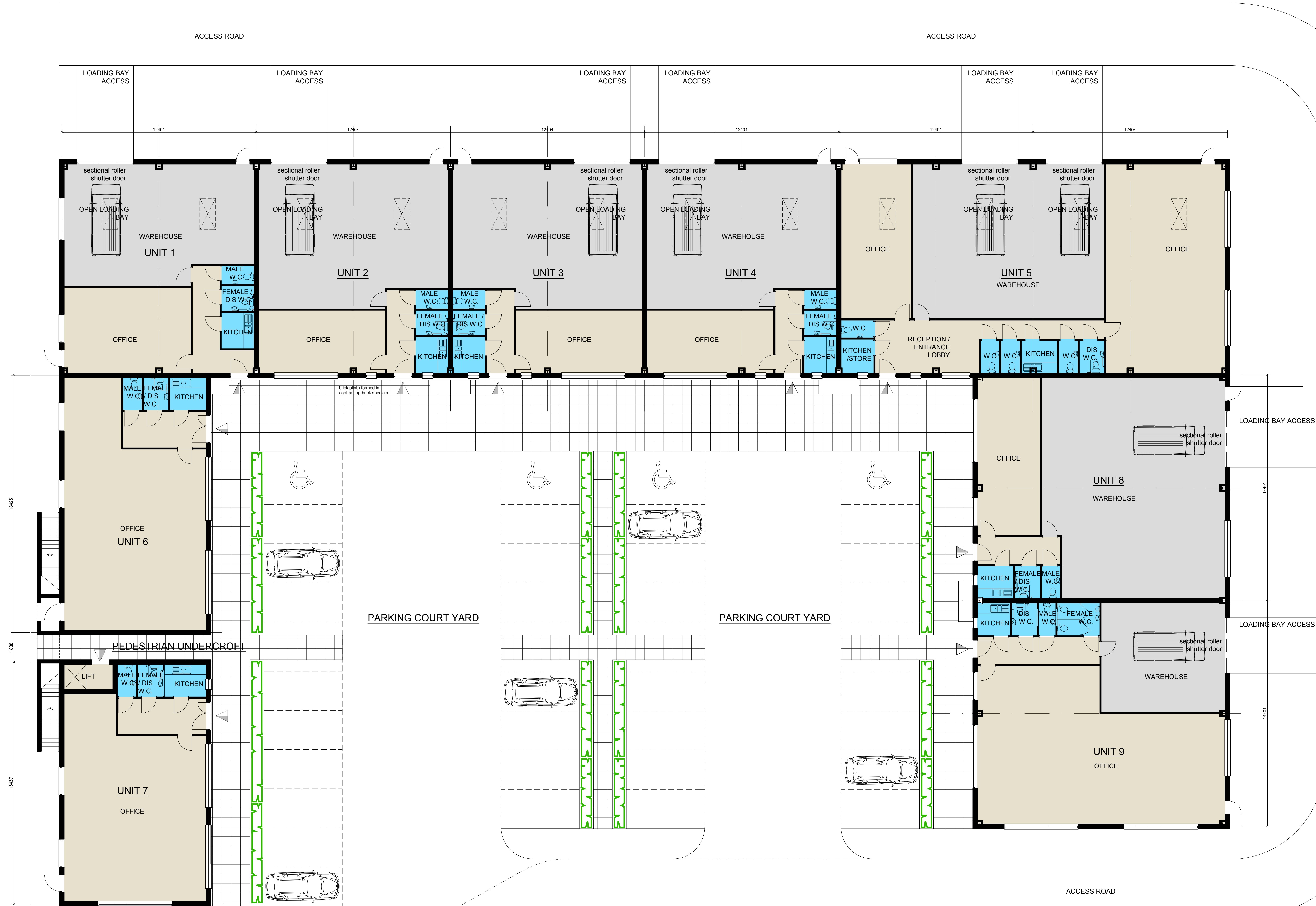
PROPOSED GROUND FLOOR PLAN 1:100 TOTAL GROSS INTERNAL AREA 2032.6M 2 OR 21,878SQ FT
